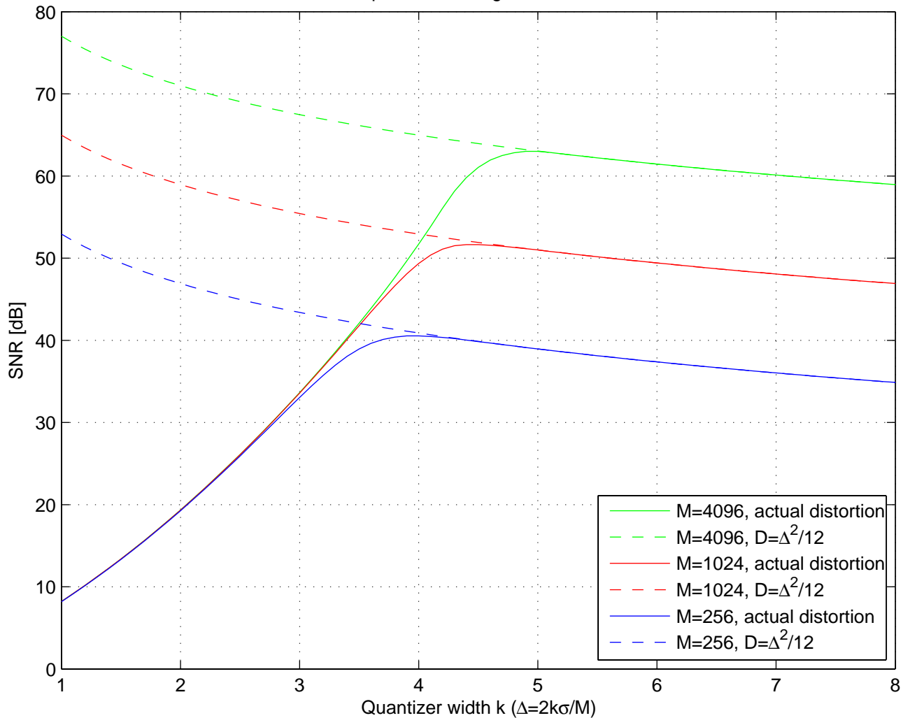
Uniform quantization of gaussian distribution
